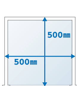
型番: FFP-HSS-55 W500×H500×D75 (mm)
